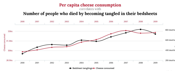
Figure 3.1: Bad Correlation v Causation Example
