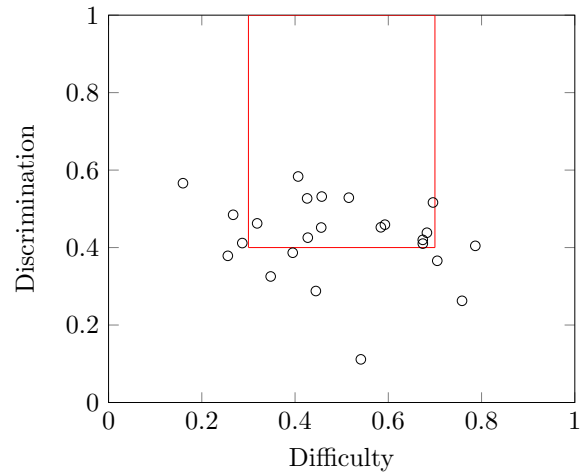
Figure C.3: 2012 Forced-rank Steadiness
