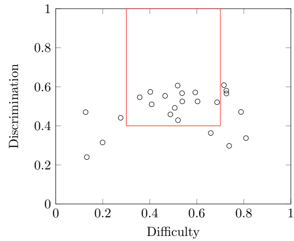
Figure C.5: 2013 Forced-rank Dominance
