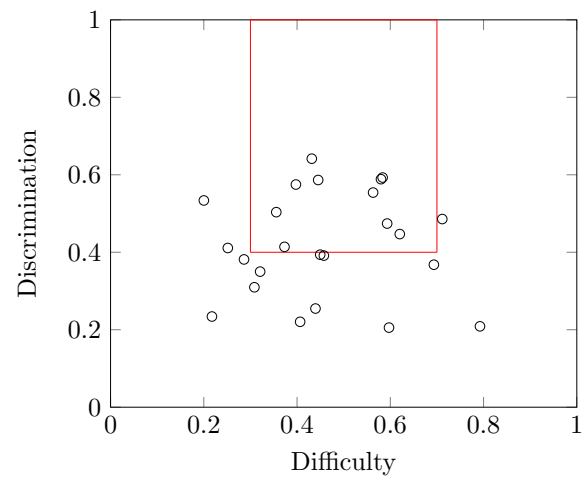
Figure C.6: 2013 Forced-rank Influence
