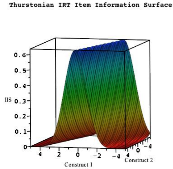
Figure 12.2: Generic Item Information Surface for Thurstonian IRT Model
