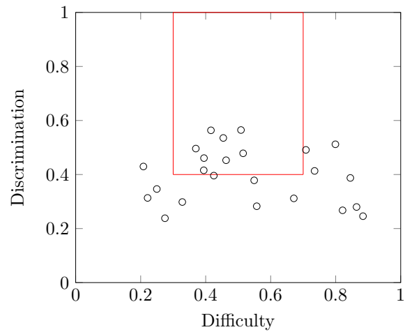
Figure C.4: 2012 Forced-rank Compliance
